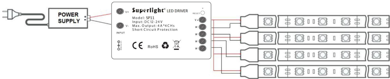
Application Circuit of SP11: single color
