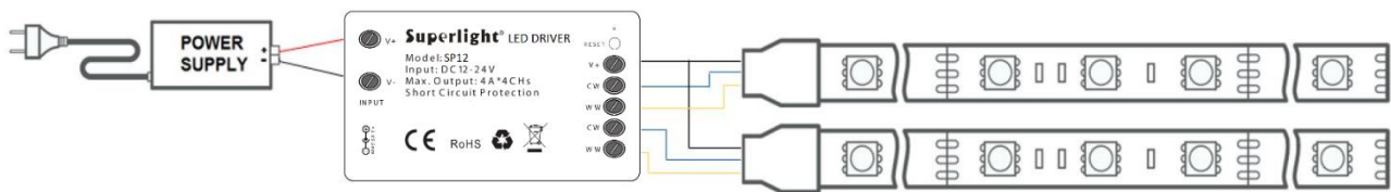
Application Circuit of SP12: CW+WW
